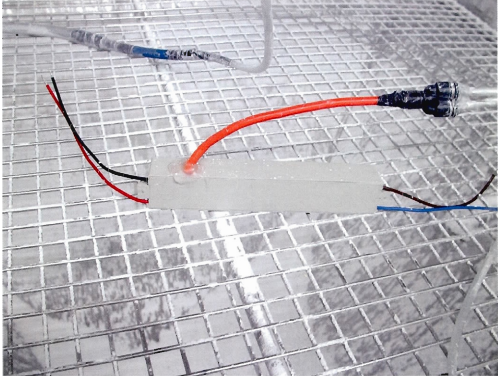
IP6X Test
